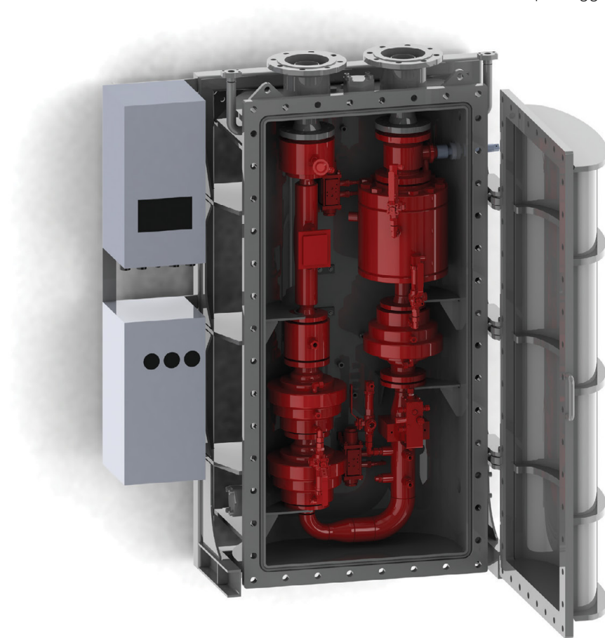
HON 750 Safety shut-off valve in Regulating line for maritime applications in pressure-resistant housing
